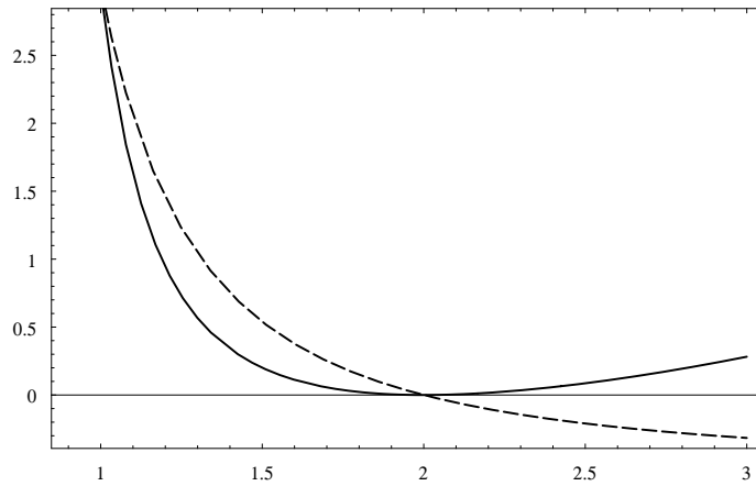
Figure 10: The value of \gamma^2 \sigma^4 - 1 , plotted as a function of the distribution parameter a for the true ML estimator (solid) and the quasi ML estimator with \lambda = 0 (dashed). When \gamma^2 \sigma^4 - 1 < 0 , the estimator is asymptotically unstable.
