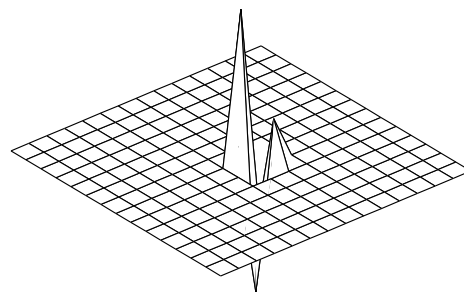
Sparsifying kernel T
