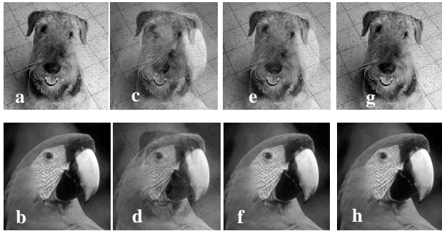
Figure 5 - Separation of synthetic mixtures. (a)-(b) Sources, (c)-(d) mixtures, (e)-(f) Reconstruction by the Farid-Adelson approach, (g)-(h) Reconstruction by SPICA with block partitioning.
