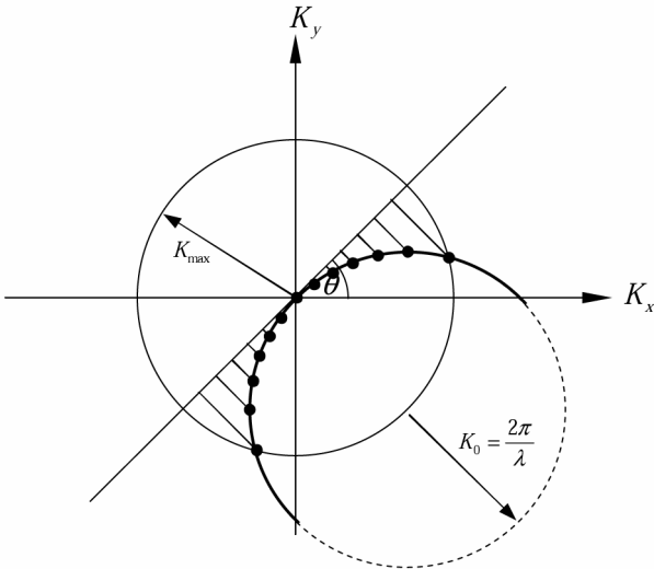
Figure 2. Illustration of the Fourier Diffraction Theorem.
