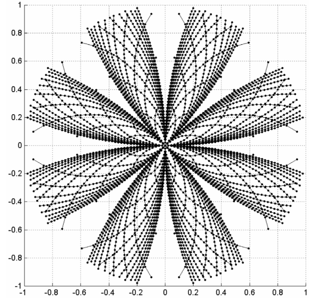
Figure 3. k-space sampling (spatial frequency is normalized to K_{\max} ).
